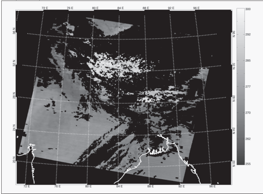
Atmospheric Temperature at 500 hPa
