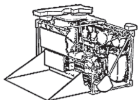
AIRS
