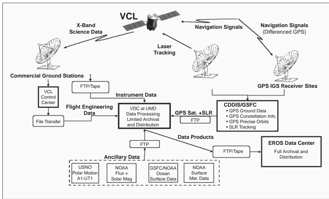
VDC System Context within the VCL Mission
